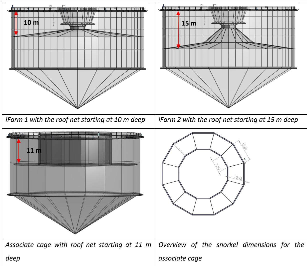
Figure 3 Technical specifications and information for each of the iFarm and associate cages utilised in Phase 1 of the iFarm project at the Cermaq Norway AS facility, Martnesvika.
